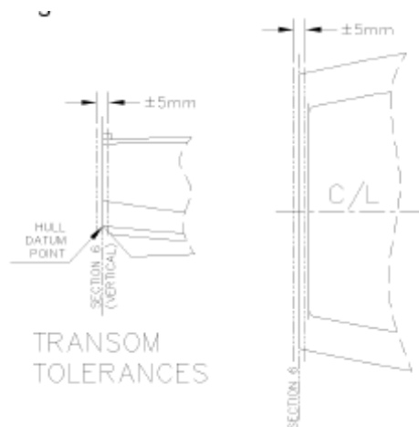
D.5.1 (b) – TRANSOM SURFACE
