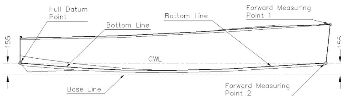
D.2.3.1 HULL DATUM POINTS DIAGRAM
